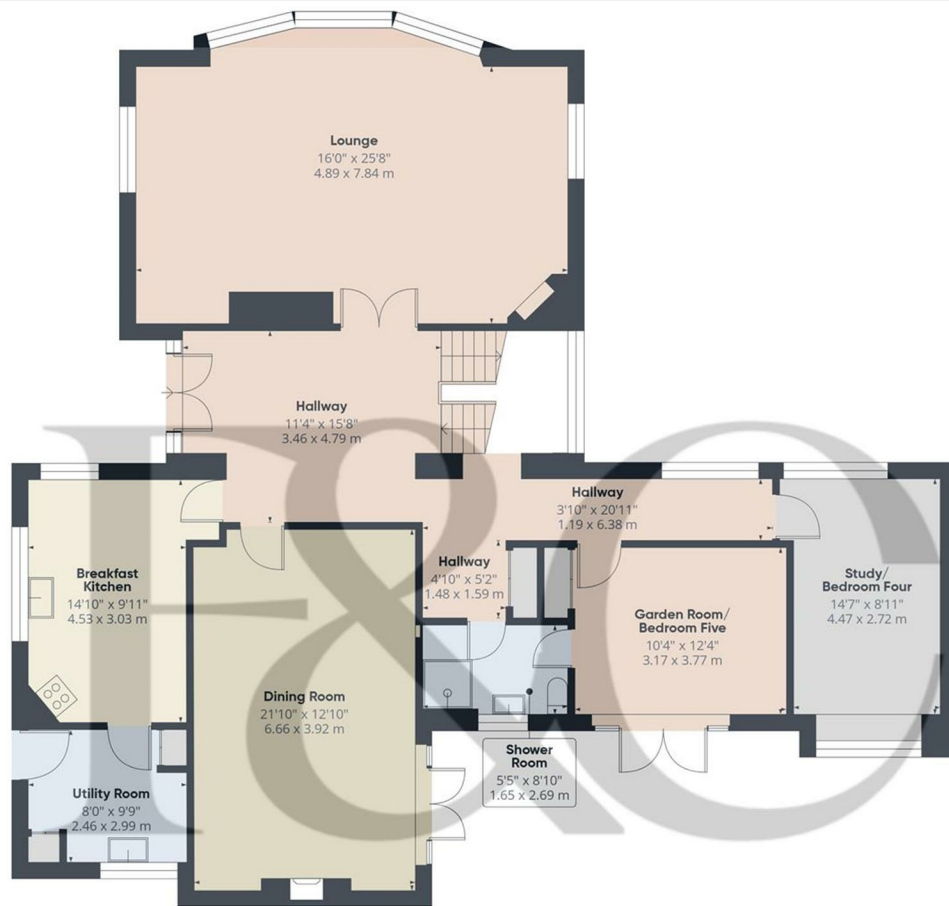
Floor 1 Building 1
