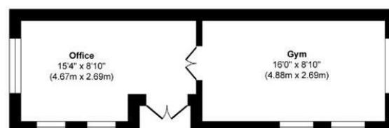
Outbuilding Approximate Floor Area 266 sq.ft (24.71 sq.m)
