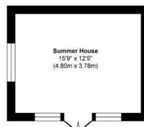
Outbuilding Approximate Floor Area 196 sq.ft (18.21 sq.m)
