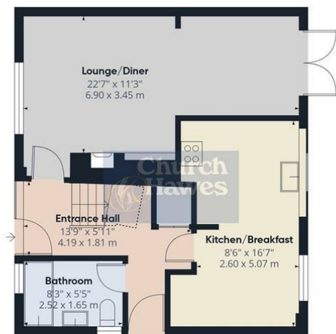
Floor 0 Building 1
