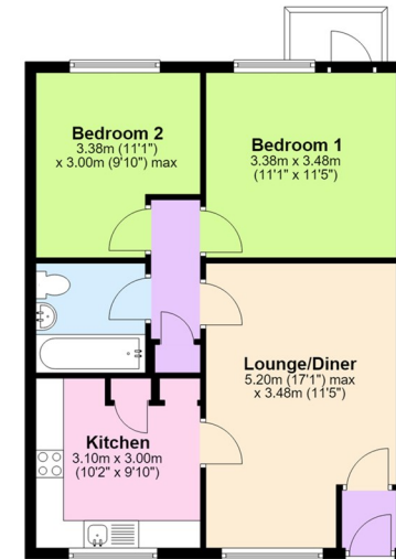
Floor Plan Approx. 56.3 sq. metres (605.6 sq. feet) (excluding Balcony)
