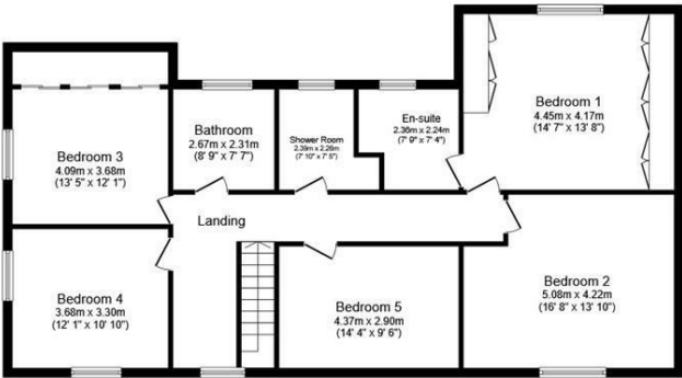
First Floor Floor area 115.8 sq.m. (1,247 sq.ft.)
