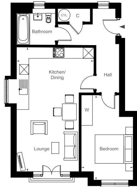
First Floor (plots 70 & 71)
