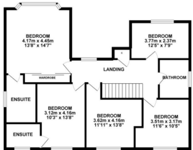
1ST FLOOR 90.61 sq. m. ( 975.36 sq. ft. )
