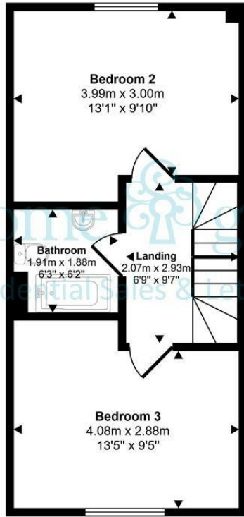
First Floor Approx 37 sq m / 396 sq ft
