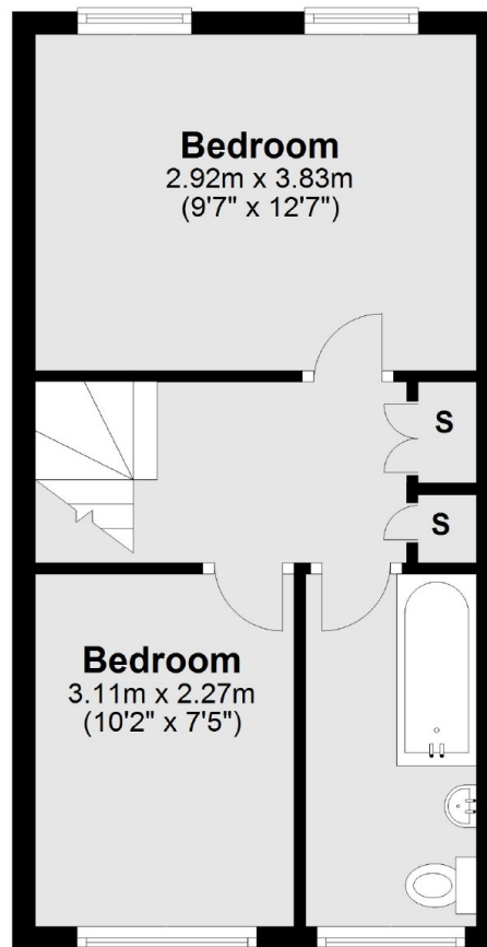
Third Floor
