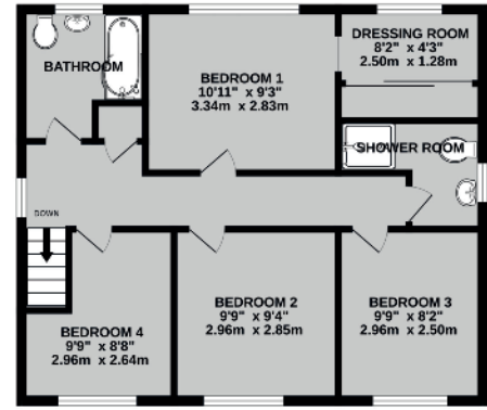
1ST FLOOR 581 sq.ft. (54.0 sq.m.) approx.
