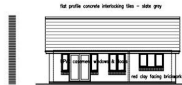
Rear elevation proposed N 1:100
