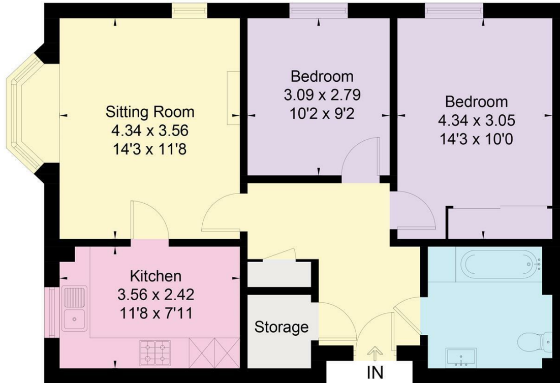
First Floor
