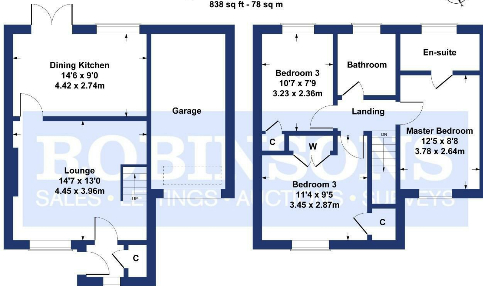
GROUND FLOOR
