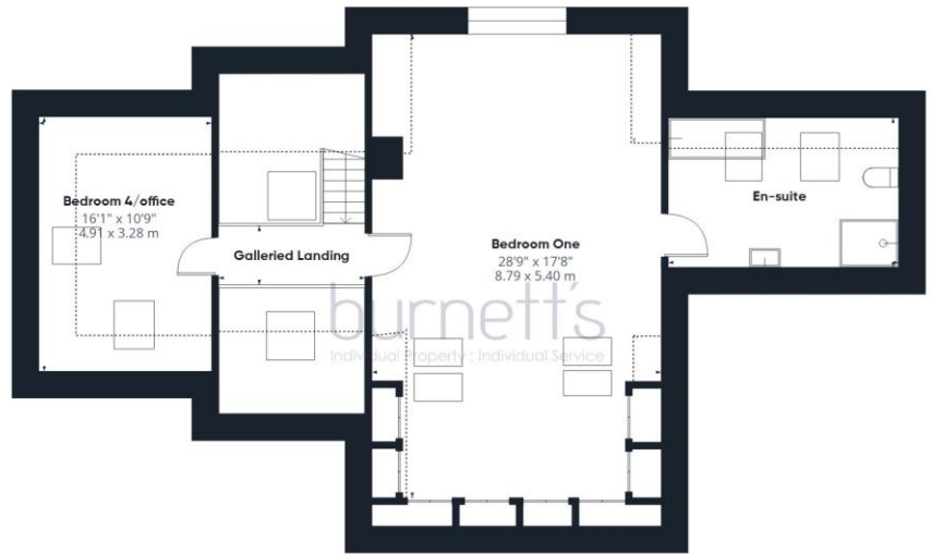
Floor 1 Building 1
