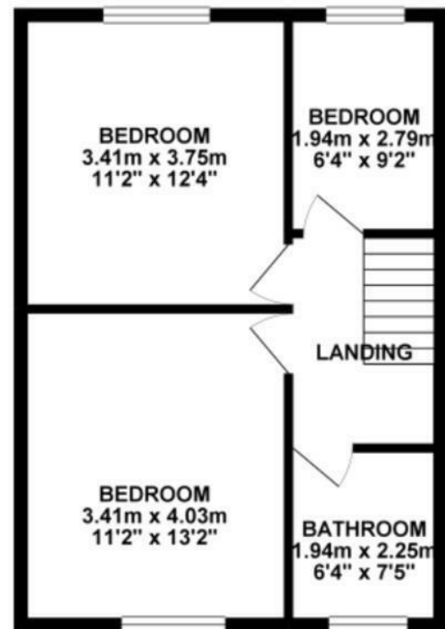
1ST FLOOR 41.57 sq. m. ( 447.48 sq. ft. )
