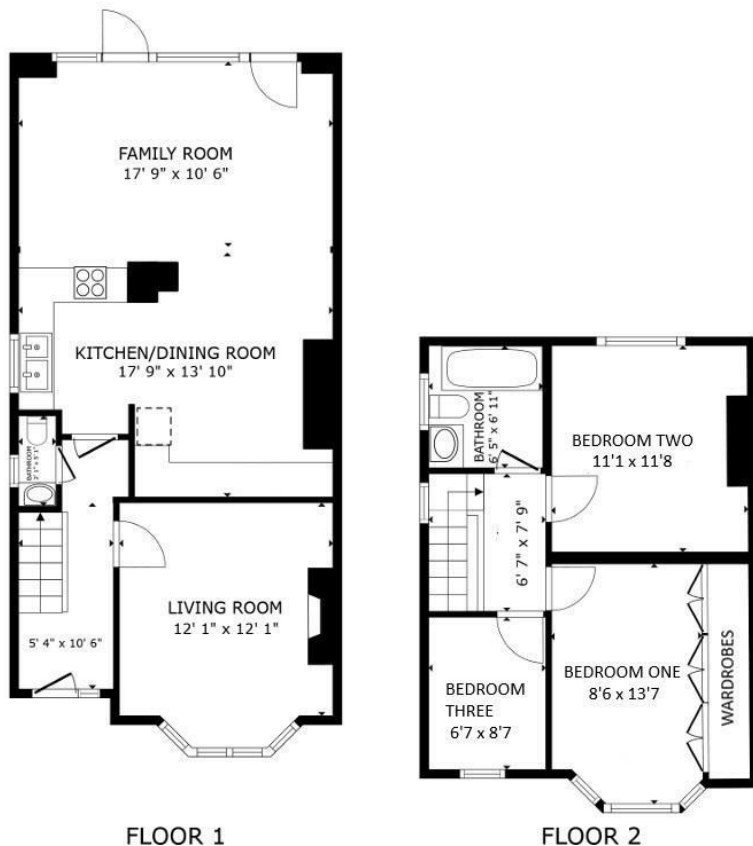
FLOOR 1
