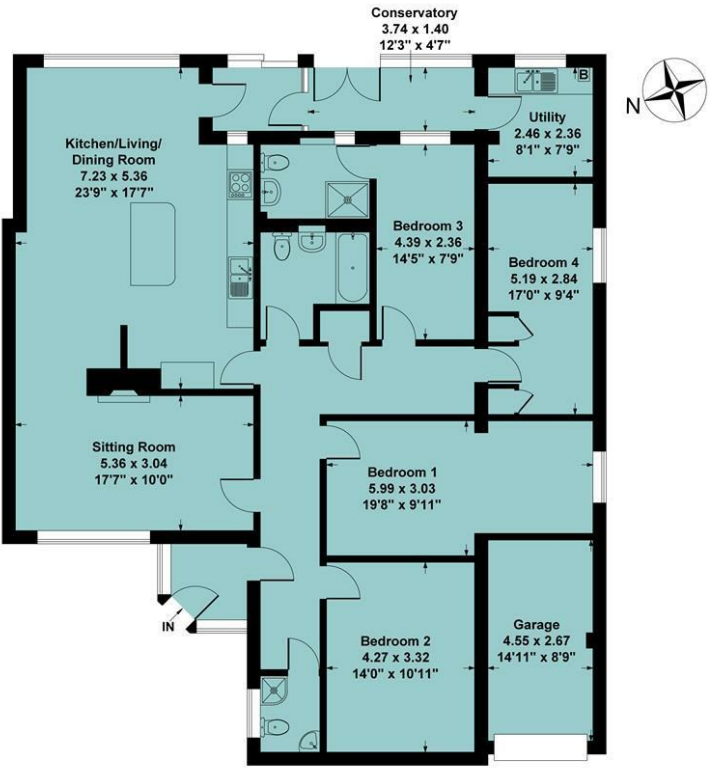
Floor Plan Floor Plan Approx Area = 162.46 sq m / 1749 sq ft Garage Approx Area = 10.66 sq m / 115 sq ft Total Area = 173.12 sq m / 1864 sq ft Measurements are approximate, not to scale, illustration is for identification purposes only. www.focuspointhomes.co.uk
