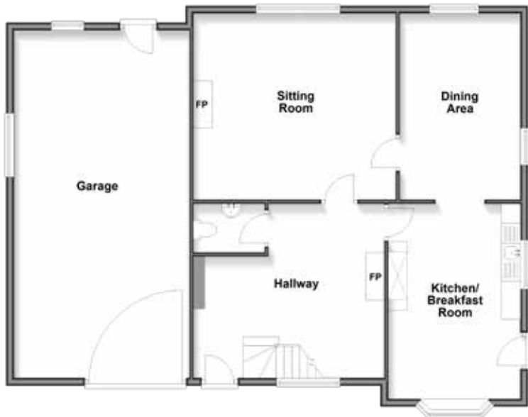
Ground Floor Approx. 128.7 sq. metres (1385.7 sq. feet)
