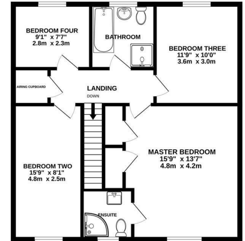
1ST FLOOR 733 sq.ft. (68.1 sq.m.) approx.
