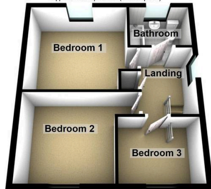
First Floor Approx. 39.0 sq. metres (419.5 sq. feet)
