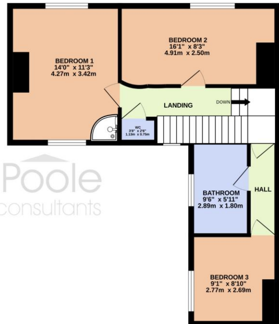
1ST FLOOR 526 sq.ft. (48.9 sq.m.) approx.
