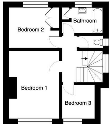
First Floor Floor Area: 45.8 m 2 ... 493 ft 2
