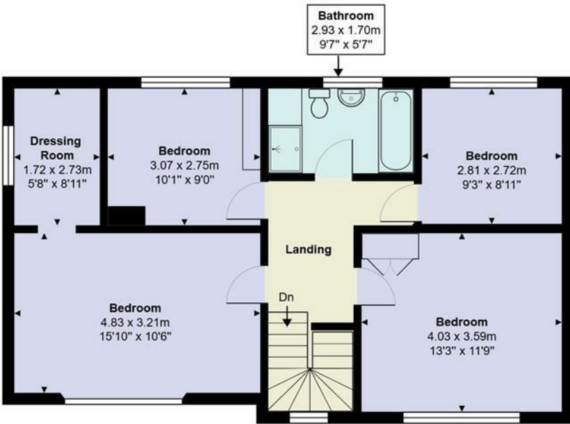
First Floor Area: 69.1 m 2 ... 743 ft 2
