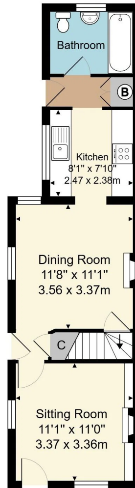
Ground Floor
