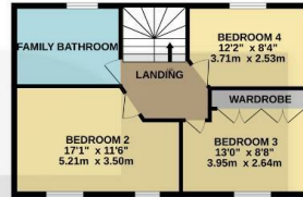
1ST FLOOR
