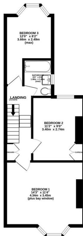
1ST FLOOR 417 sq.ft. (38.8 sq.m.) approx.
