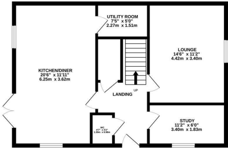
GROUND FLOOR 625 sq.ft. (58.0 sq.m.) approx.
