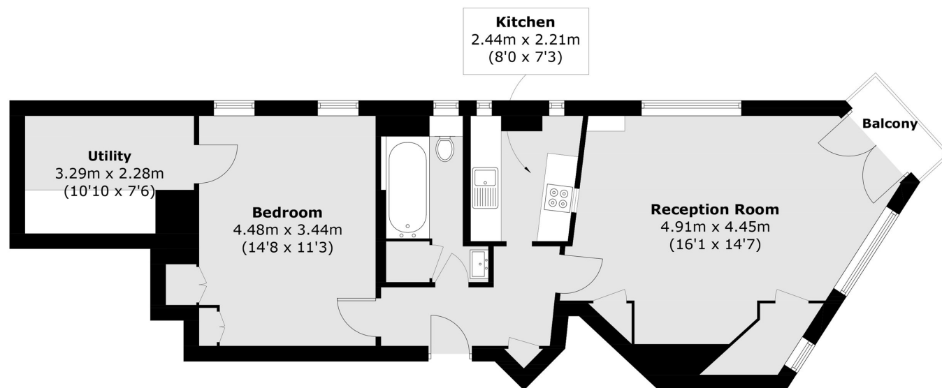
Fourth Floor
