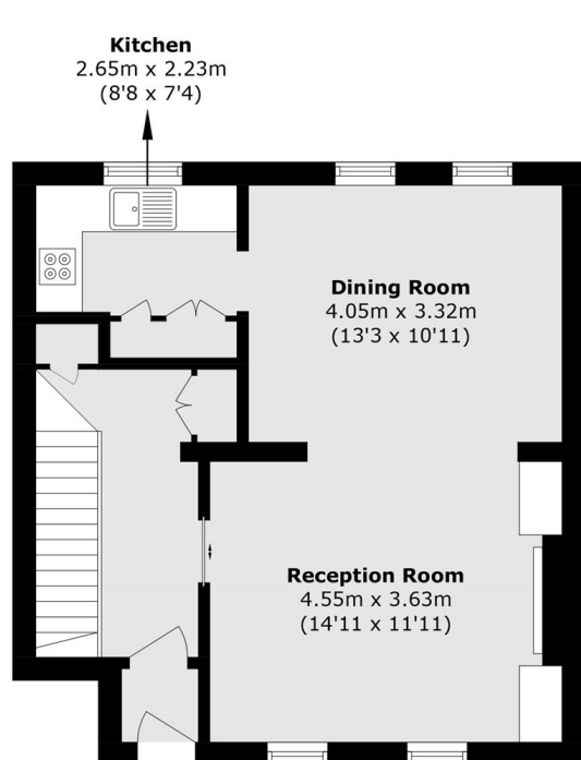
Raised Ground Floor
