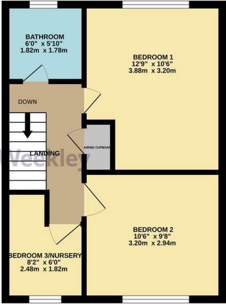
1ST FLOOR 369 sq.ft. (34.2 sq.m.) approx.
