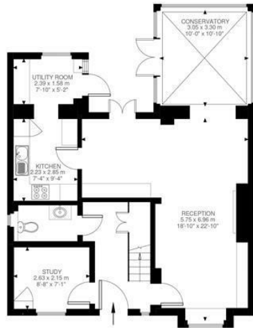
Ground Floor 768 ft²
