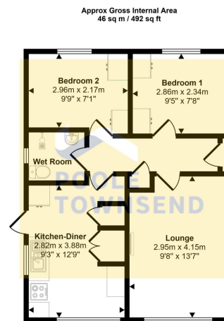
Floorplan
