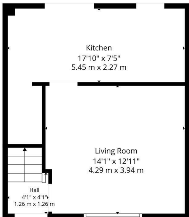
1st Floor
