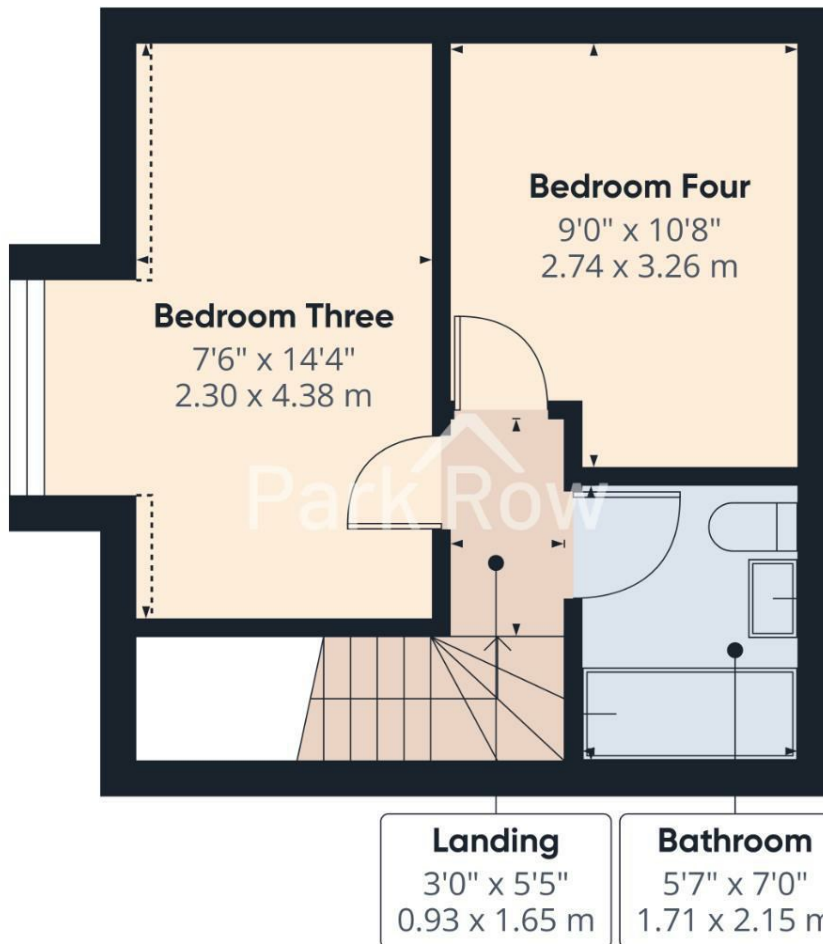
Floor 2 Building 1
