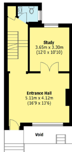
GROUND FLOOR
