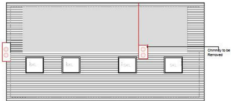
Proposed Roof Plan Scale 1:100
