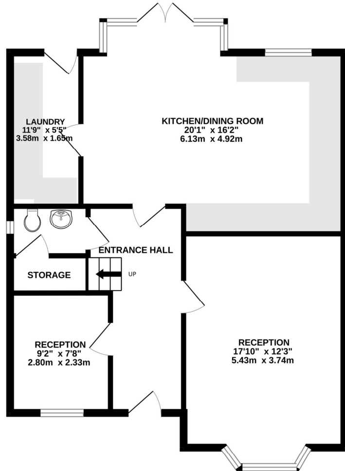
GROUND FLOOR 764 sq.ft. (70.9 sq.m.) approx.
