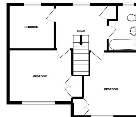
1ST FLOOR 503 sq.ft. (46.7 sq.m.) approx.
