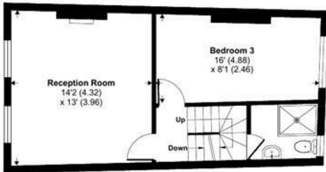
SECOND FLOOR
