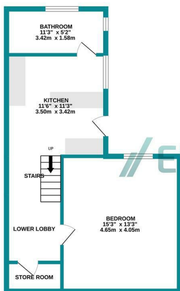
LOWER GROUND FLOOR 485 sq.ft. (45.1 sq.m.) approx.
