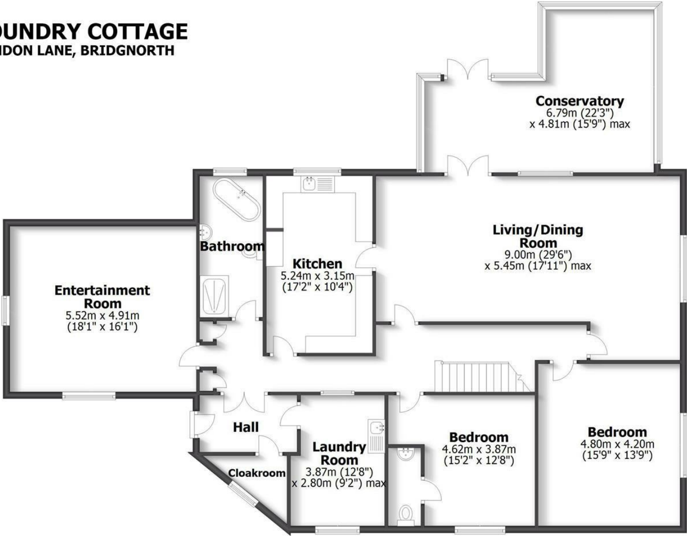
Ground Floor
