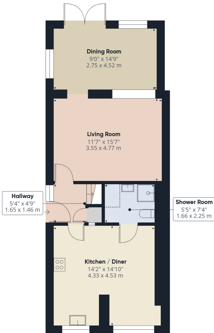
Floor 0 Building 1
