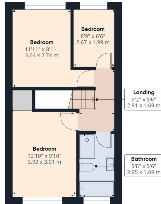
Floor 1 Building 1
