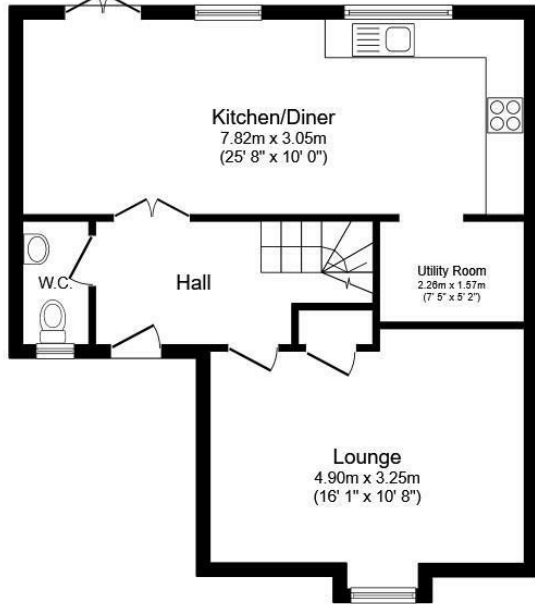
Ground Floor Floor area 56.8 sq.m. (612 sq.ft.)
