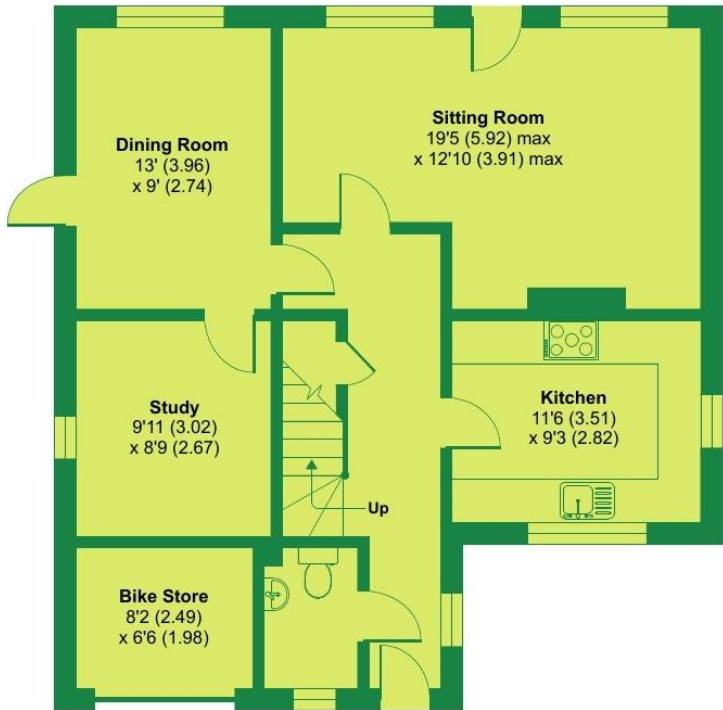
GROUND FLOOR
