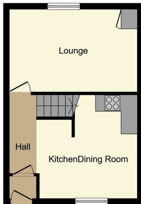
Ground Floor Floor area 32.5 sq.m. (350 sq.ft.)
