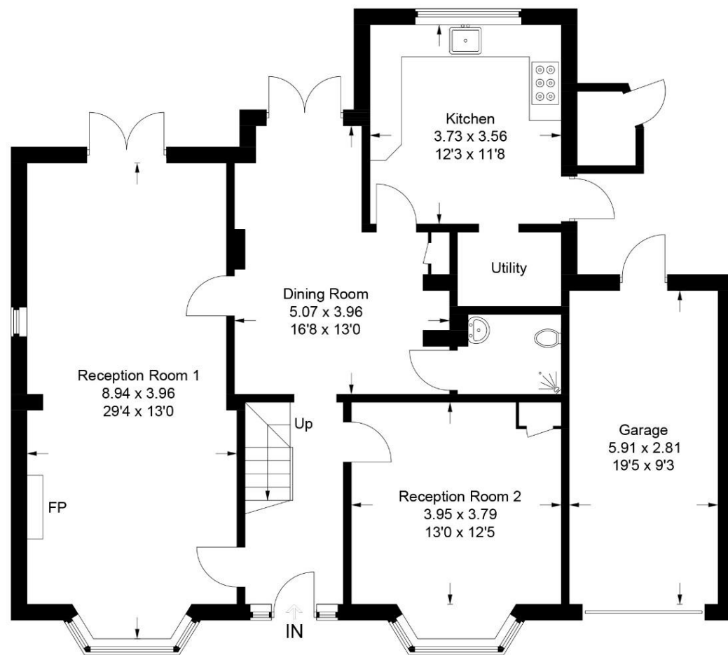
Ground Floor
