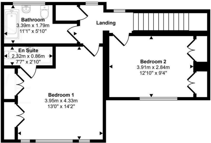
First Floor Approx 48 sq m / 516 sq ft
