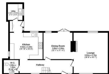
Ground Floor Floor area 85.5 sq.m. (920 sq.ft.)
