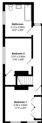
First Floor Area: 38.7 m 2 ... 416 ft 2
