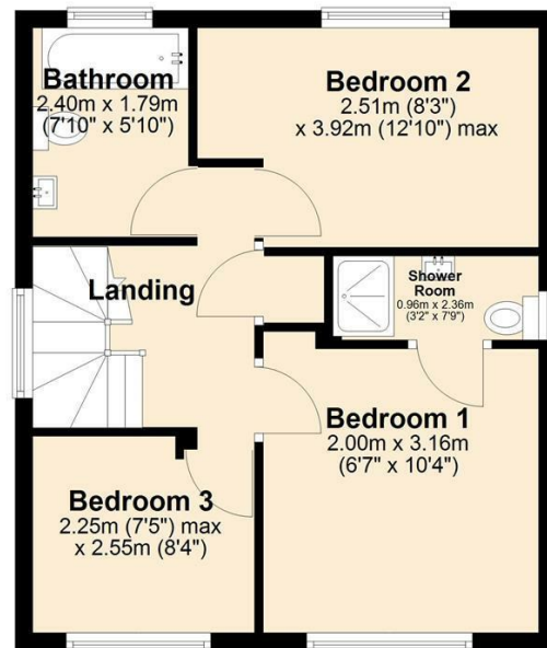
First Floor Approx. 40.1 sq. metres (431.9 sq. feet)
