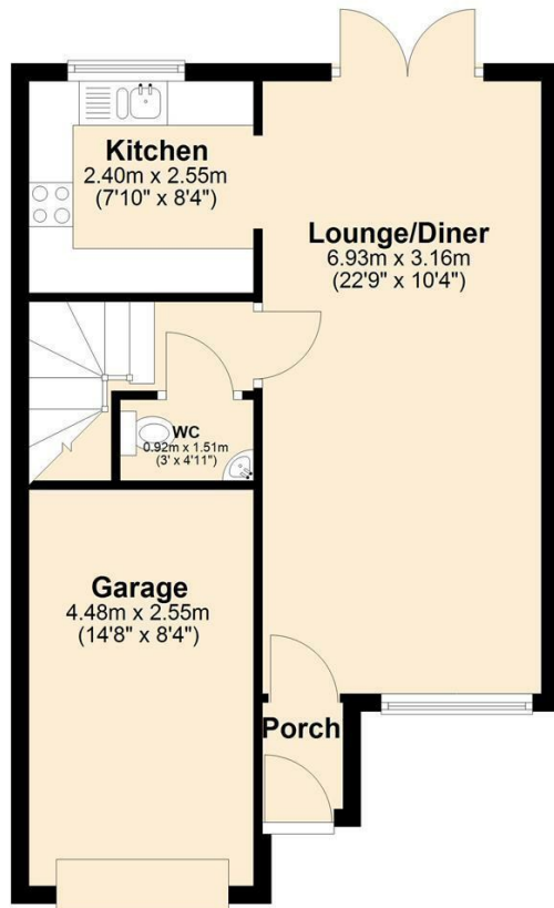
Ground Floor Approx. 47.1 sq. metres (506.7 sq. feet)
